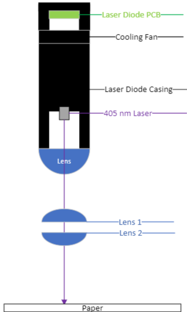
Figure 47; Laser diode controller schematic that was used in the second demo
