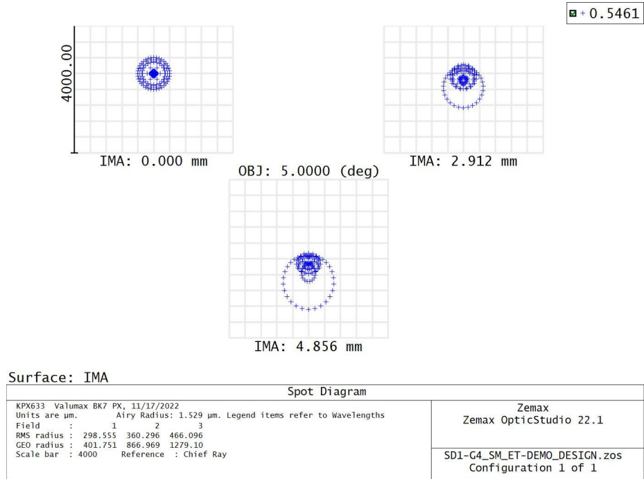
Figure 54; Final Beam Spot Patterns for On and Off-Axis Rays
