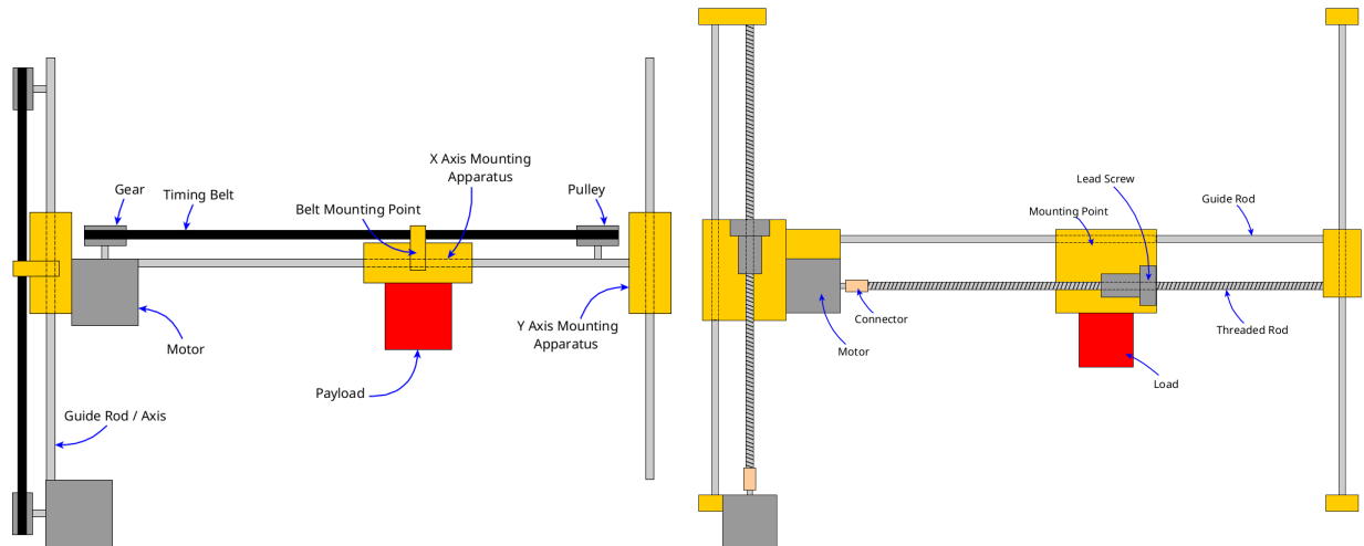
Figure 13; Conjoined Independently Driven Axis configuration for timing belts (left) and threaded rods (right)
