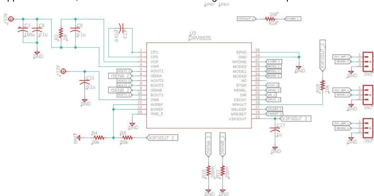
Figure 33; The DRV8825 motor controller application which was replicated from an example in the datasheet onto our design. The pin headers on the right are for selecting step resolutions.
