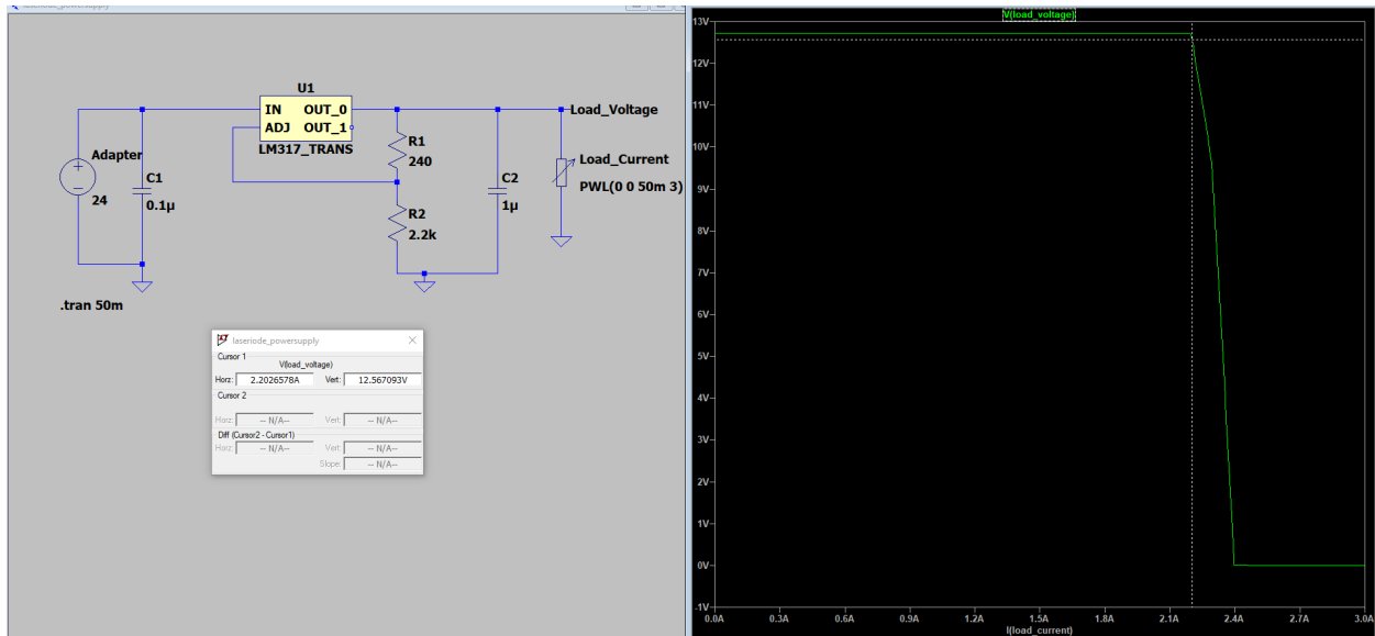
Figure 28; LM317 Adjustable Regulator output schematic and transient simulation, 12V output and 0-3A load range
