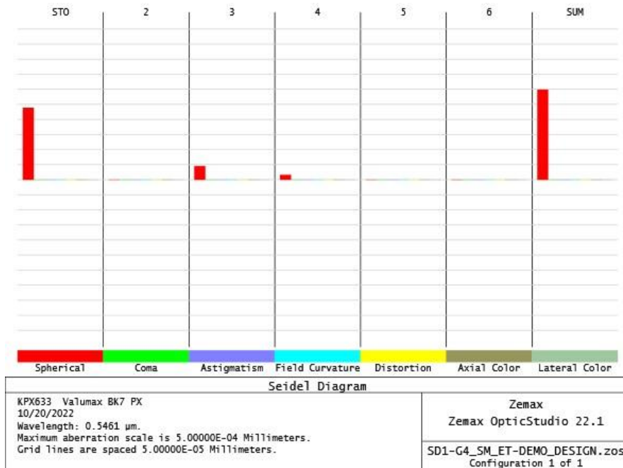
Figure 46; Zemax Seidel Diagram
