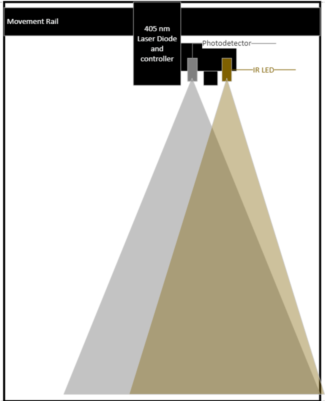
Figure 21; Diagram of how the time of flight method would work
