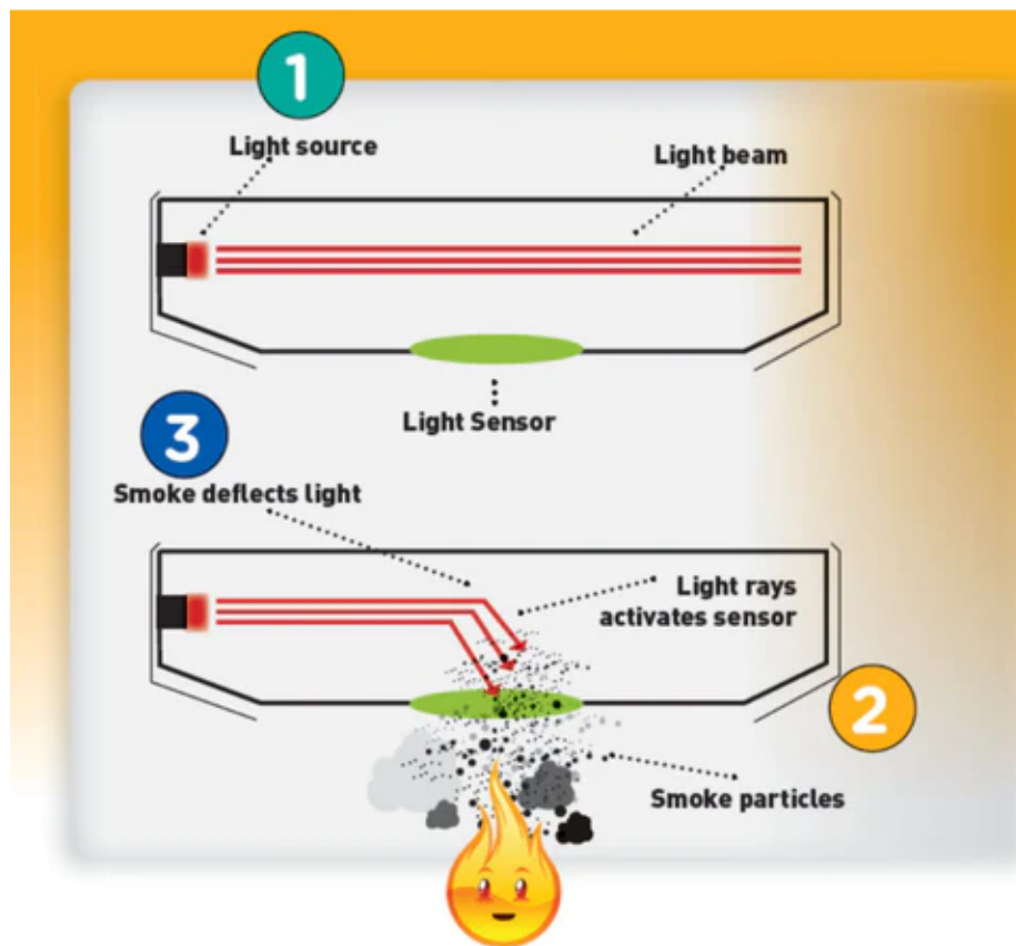
Figure 10; How an optical fire alarm works[19]
