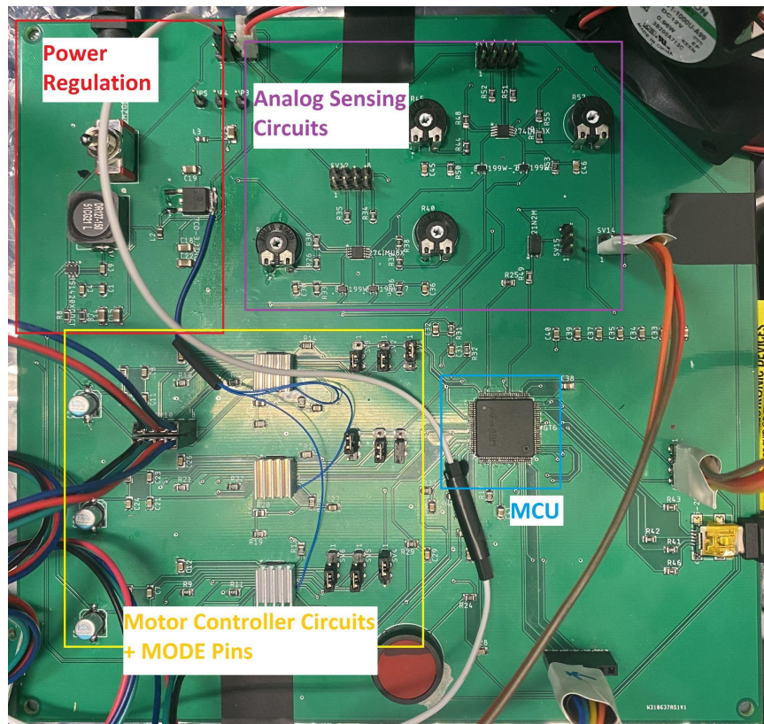
Figure 35; Fully assembled D-MILE PCB with labels and sections showing off the different subsystems on the board.
