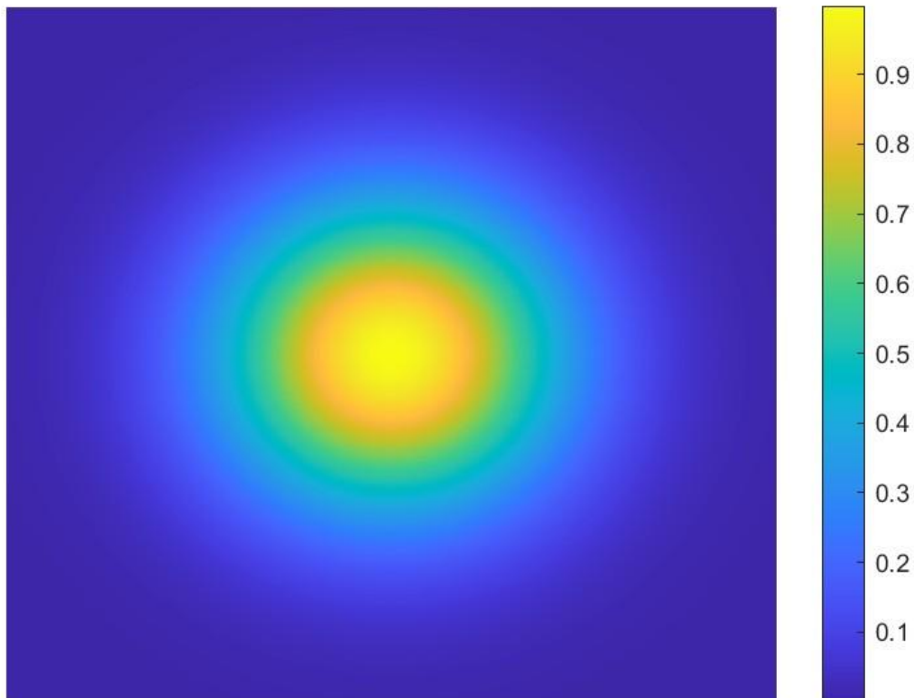
Figure 9; Intensity Graph of the Gaussian beam profile that will be used in our system
