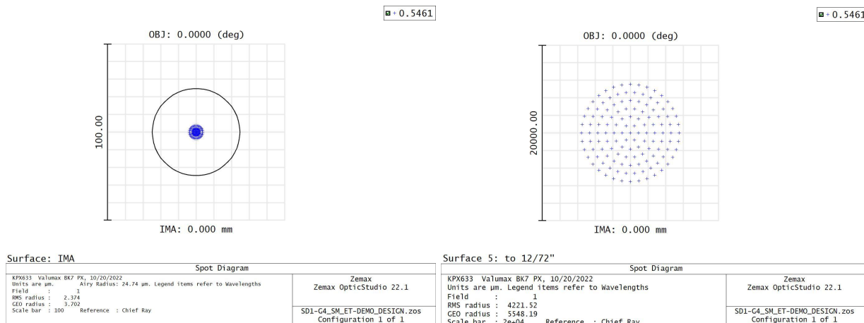
Figure 45; Spot size that Zemax calculated with the an analysis of the results
