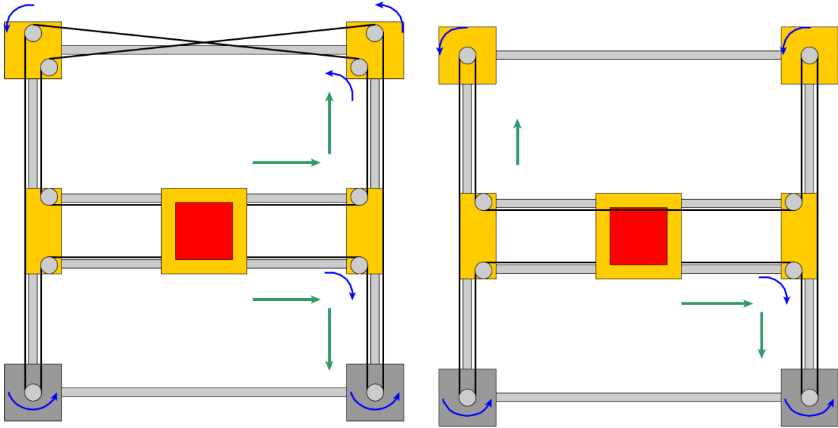
Figure 15; Tension forces (green) and Belt direction (blue) for Core-XY and H-Bot configurations when moving along the positive X-axis
