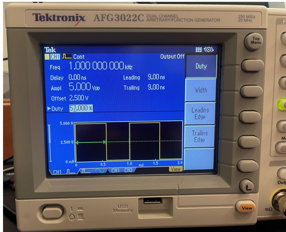
Figure 56; Function Generator Settings
