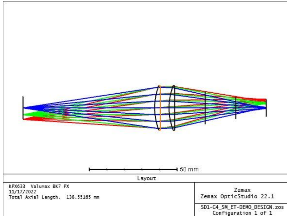
Figure 52; Beam Path for On and Off-Axis Rays for Final System
