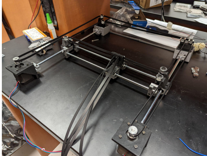
Figure 67; Prototype standalone XY gantry
