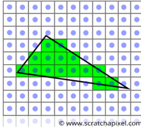
Figure 4; Rasterization example from ScratchAPixel
