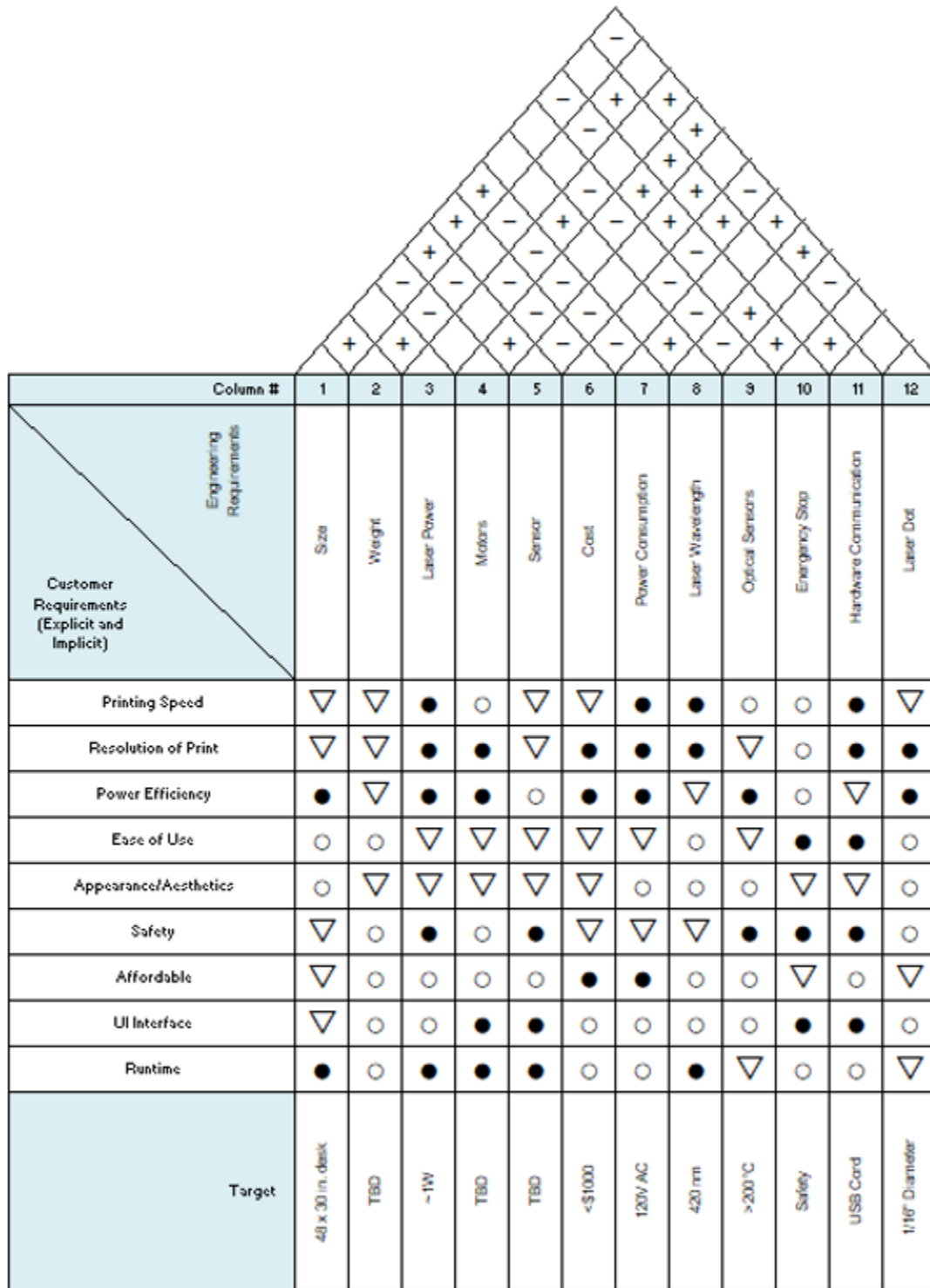
Figure 2; House of Quality
