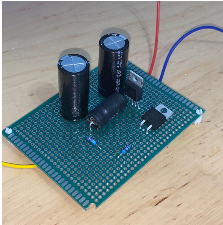
Figure 41; LM2576 Adjustable regulator with 12V output
