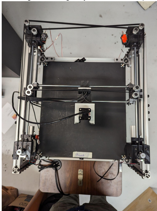
Figure 68; Final XY gantry version mounted to frame
