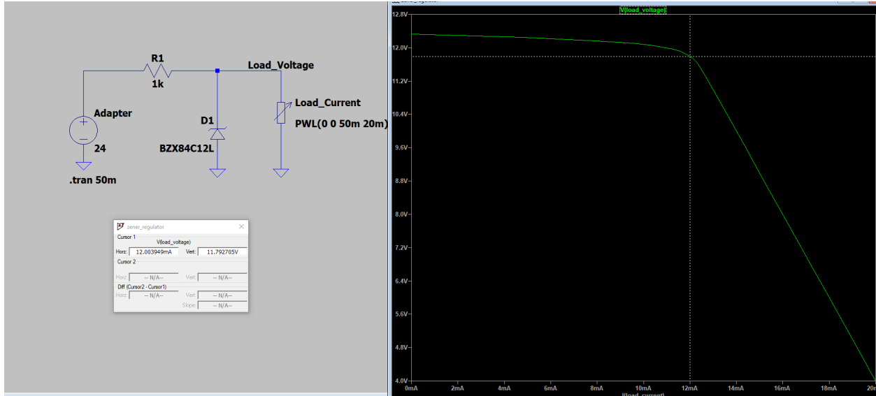
Figure 27; Zener Regulator schematic and transient simulation, 12V output and 0-20mA load range
