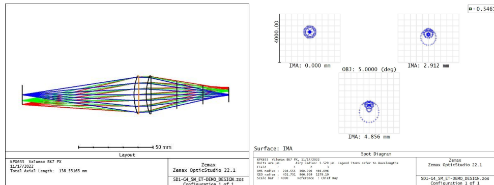
Figure 19, Lens design
