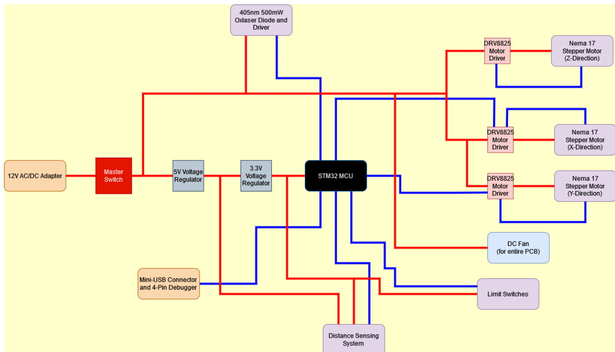
Figure 25; High-Level Design Flowchart
