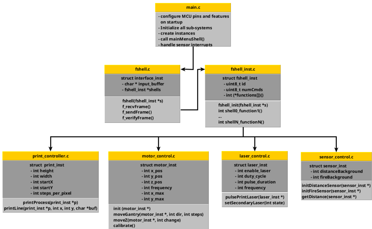
Figure 36; General firmware components and program flow
