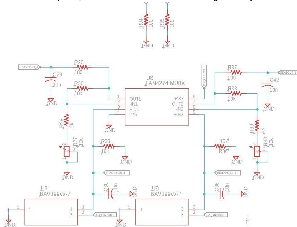
Figure 32; The distance sensing circuit used for fire detection and distance sensing. The input is the voltage change of the photodiode and its output is an analog signal ranging from 0V to 3.3V to be input into the microcontroller.
