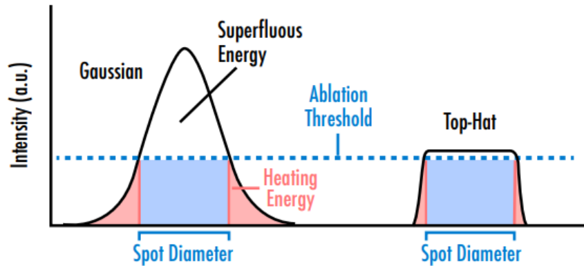
Figure 7-8; Gaussian, Flat Top, and Top-Hat beam profiles[1]
