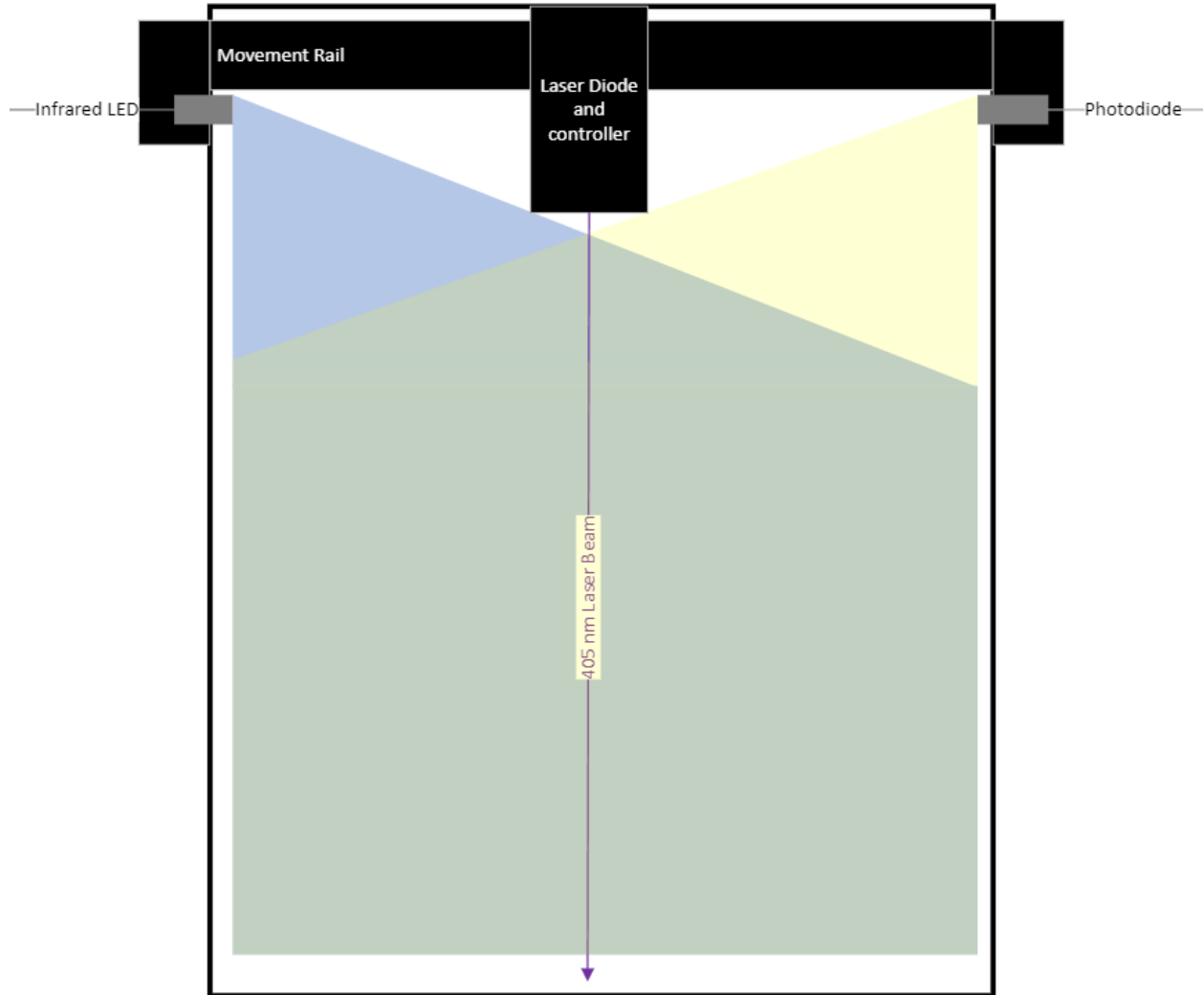
Figure 20; Schematic of how a fire safety system could be designed for our system
