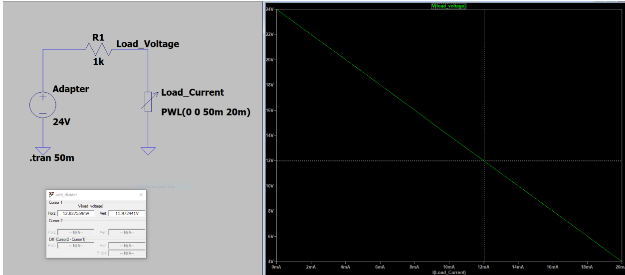
Figure 26; Voltage Divider Regulator schematic and transient simulation, variable voltage output and 0-20mA load range
