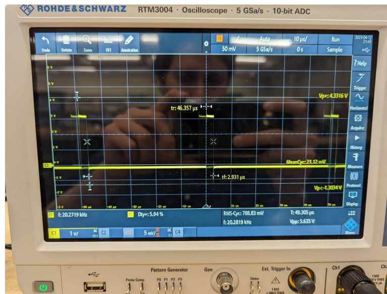
Figure 65; Oscilloscope output from laser controller of a 20 kHz 6% duty cycle PWM signal
