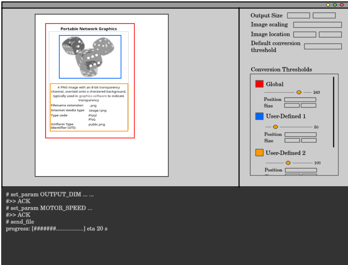
Figure 39; Planned design of GUI
