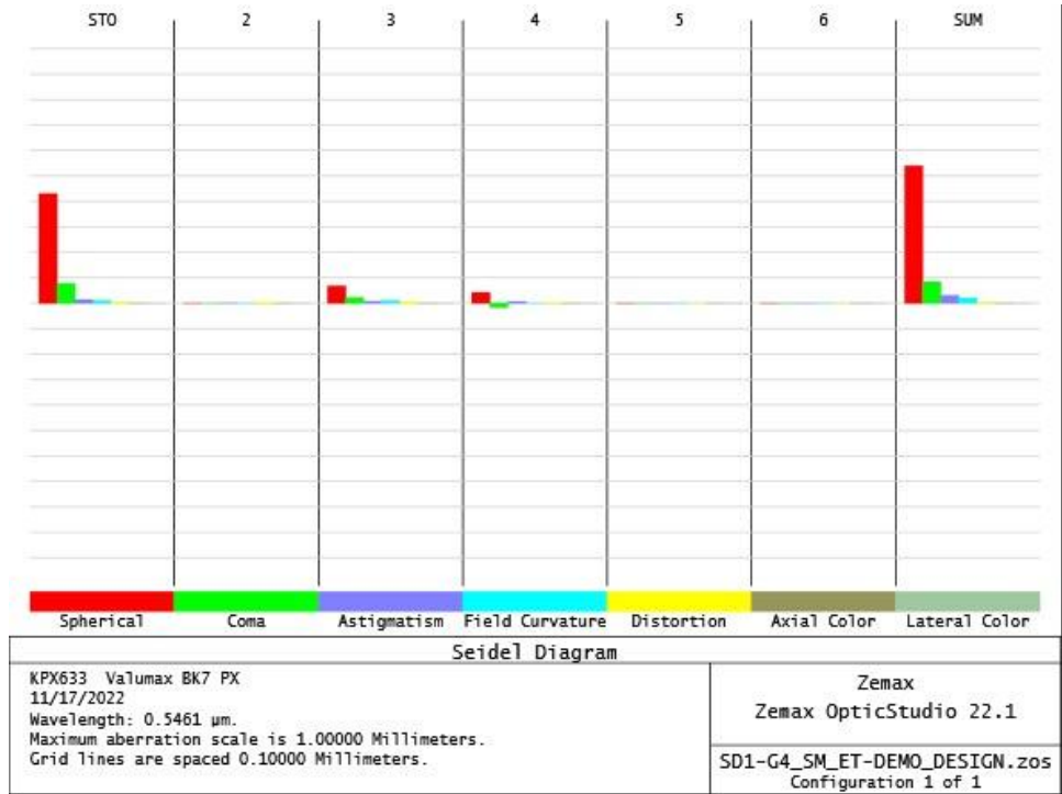
Figure 53; Final Seidel Diagram
