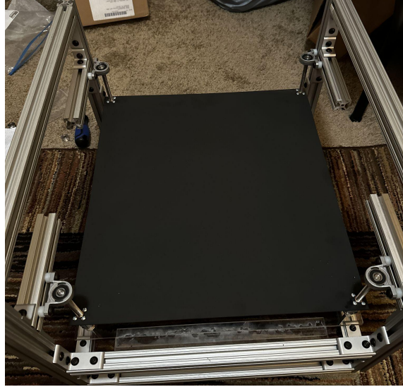
Figure 71; Z-stage of D-MILE with print bed
