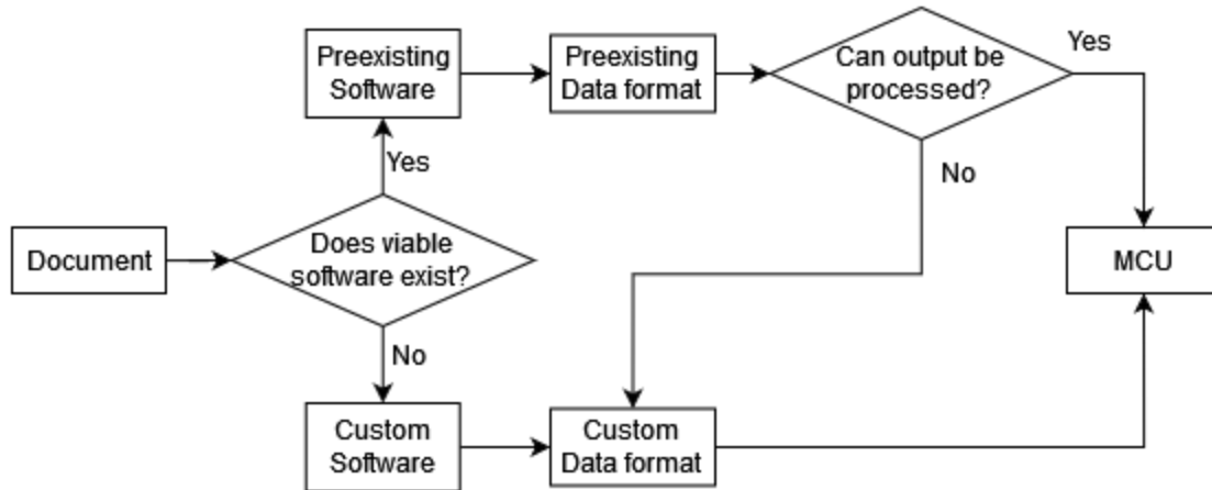
Figure 6; Decision diagram for software development
