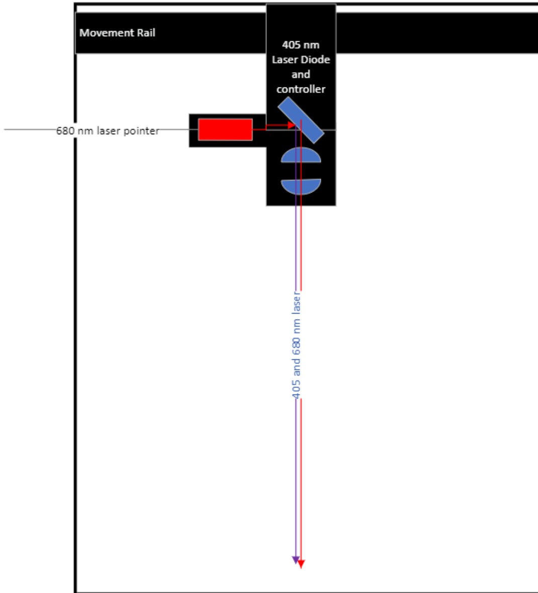
Figure 23; Optical Workspace Detection System mounting option 2
