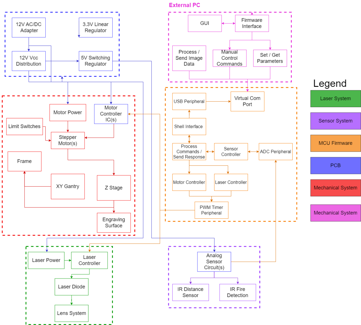
Figure 3; Subsystem block diagram and distribution of work
