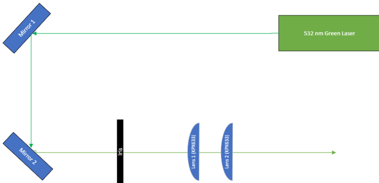
Figure 42; Schematic of the laser setup for the first demo
