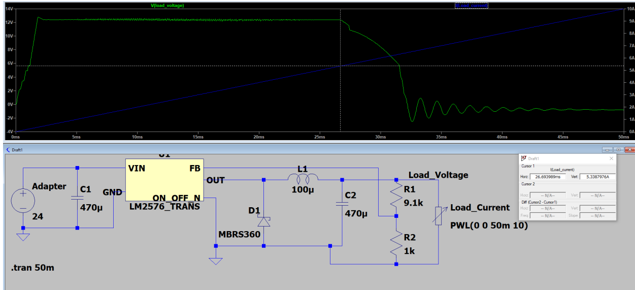
Figure 29; LM2576 Adjustable Switching Regulator schematic and transient simulation, 12V output and 0-10A load range
