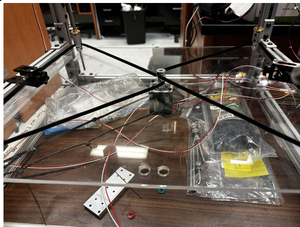
Figure 70; Z-stage movement system of D-MILE before print bed
