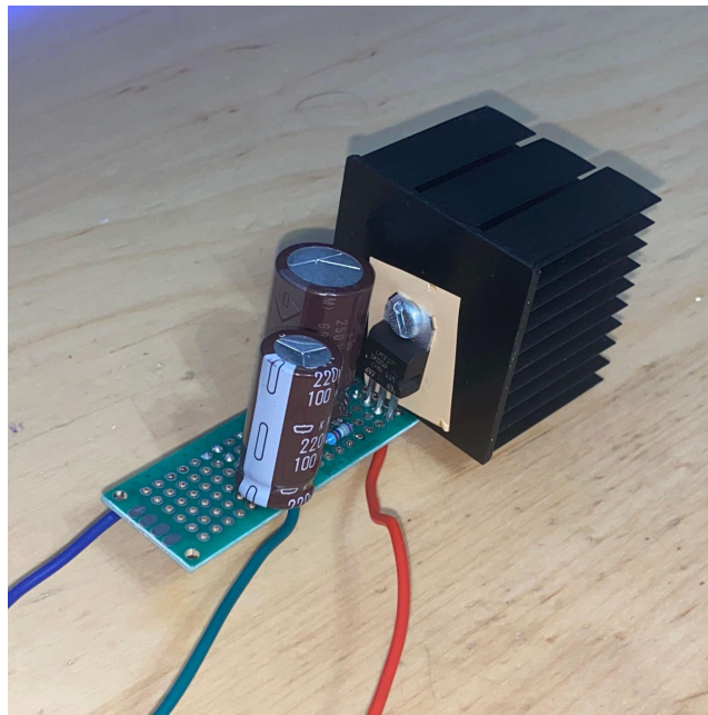
Figure 40; LM317 Adjustable Regulator prototype with 12V output
