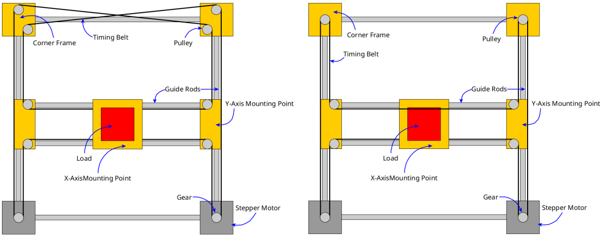
Figure 14; Core-XY belt configuration (left) and H-Bot belt configuration (right)
