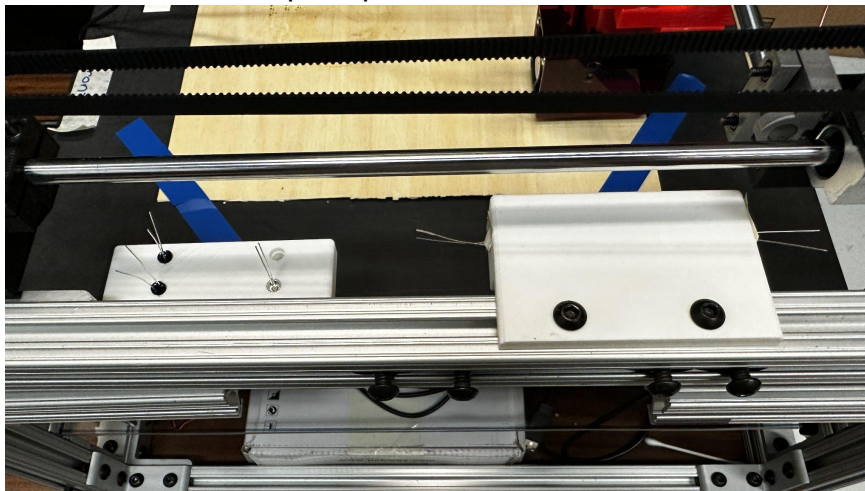
Figure 59; Distance sensor and Fire Detection system mounted to the frame of D-Mile
