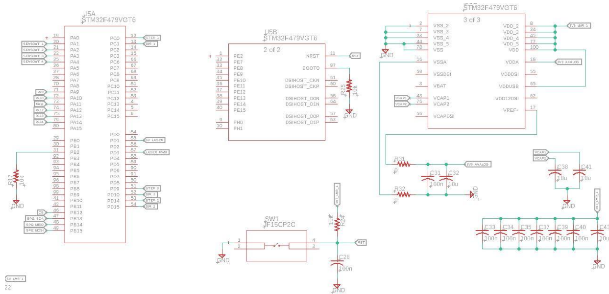
Figure 34; The STM32 microcontroller connections schematic as used on our PCB. Data connections are shown, as well as power and a reset button.
