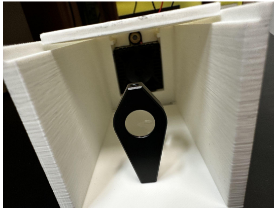
Figure 63; 650nm laser pointer inside the old laser mount
