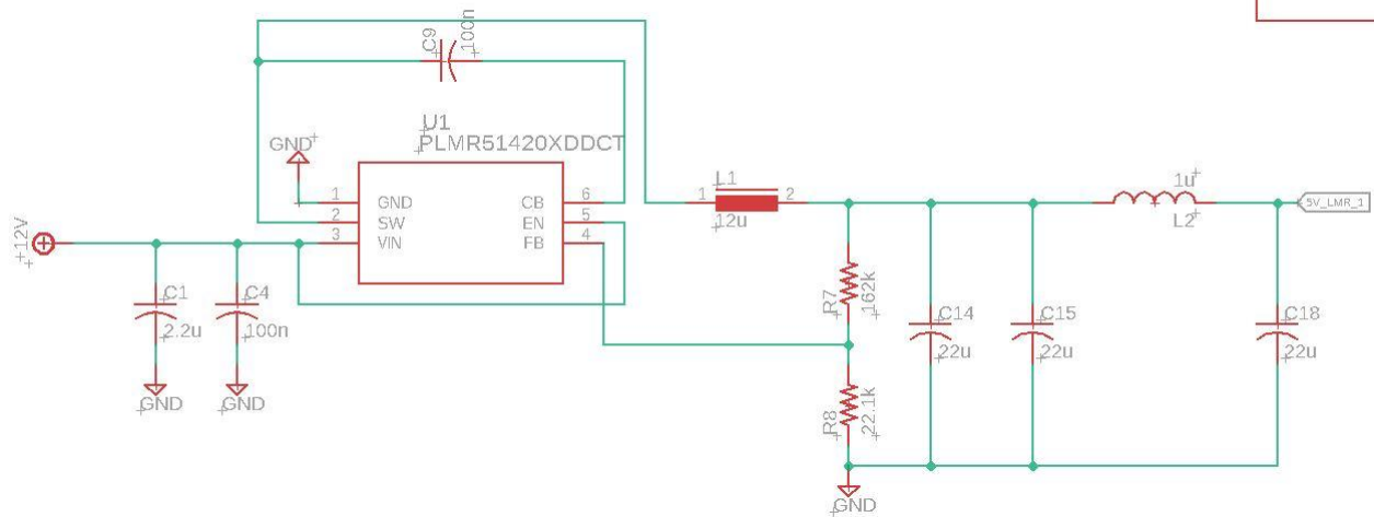
Figure 30; LMR51420 Adjustable Switching regulator schematic as used on our PCB design
