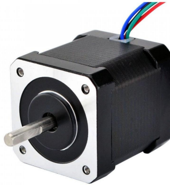
Figure 12; The Nema 17 Stepper motor that will be used in our design, for both X and Y axis movement of the laser diode.
