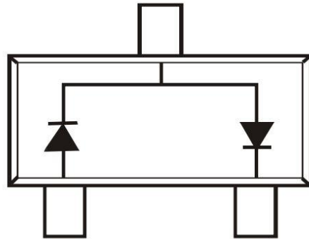
Figure 17; The BAV199 footprint and schematic taken from its datasheet
