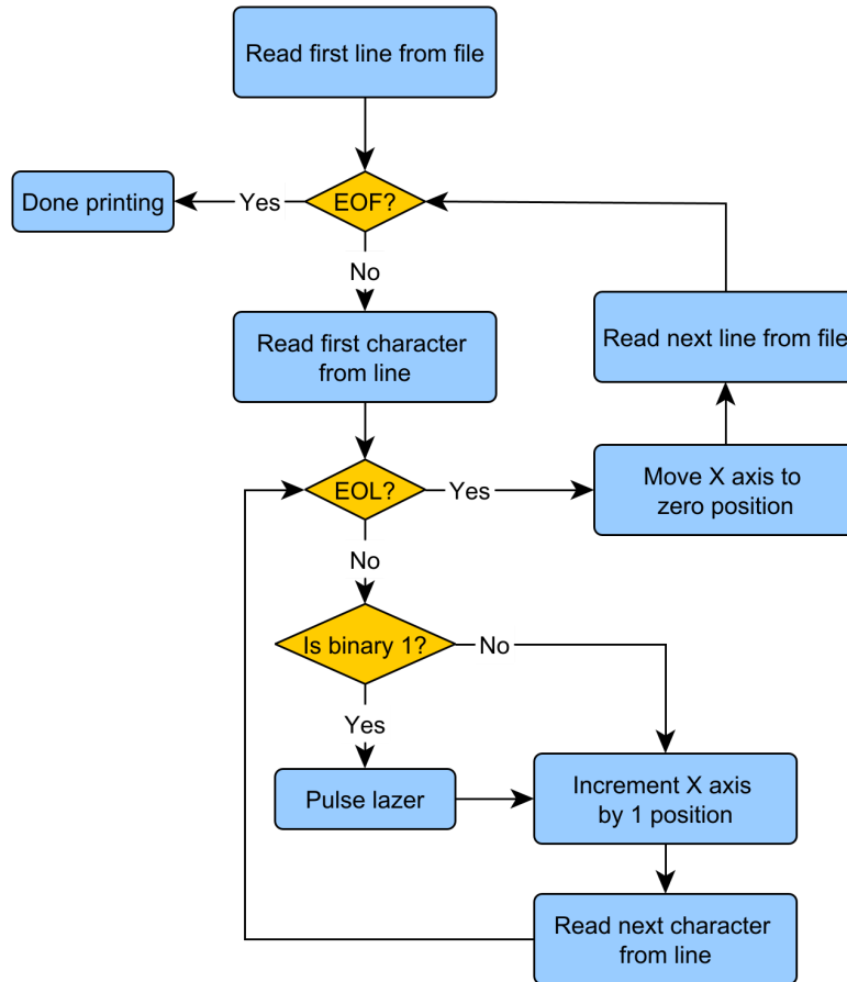
Figure 37; Printing process in MCU firmware
