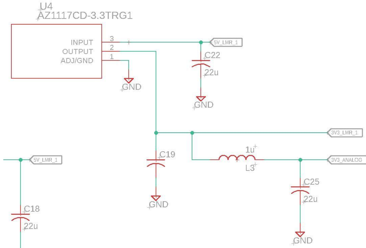
Figure 31; The AZ1117 3.3V Linear Dropout Regulator schematic as used on our PCB design, including a branch with a filter for 3.3V analog use
